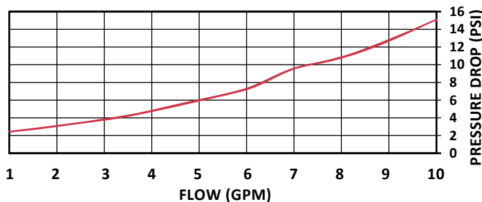
ICVN NOZZLE
