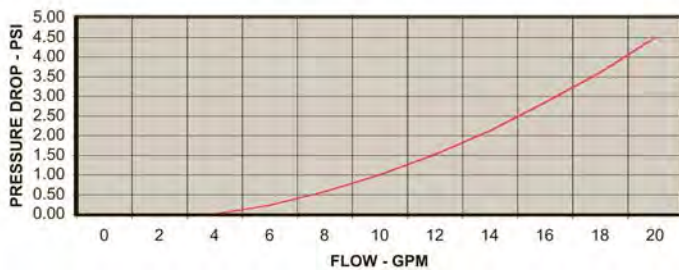
C720-3/4 SWIVEL
